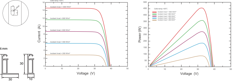
Current-Voltage & Power-Voltage Curves (SKT455M10-108D4)
